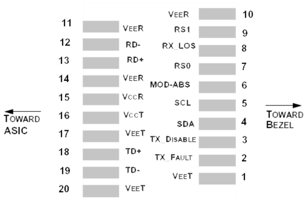
Figure 3,pins view
