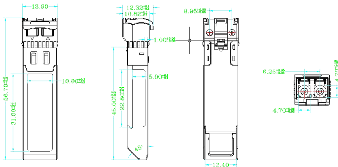
Figure 4,mechanical dimension
