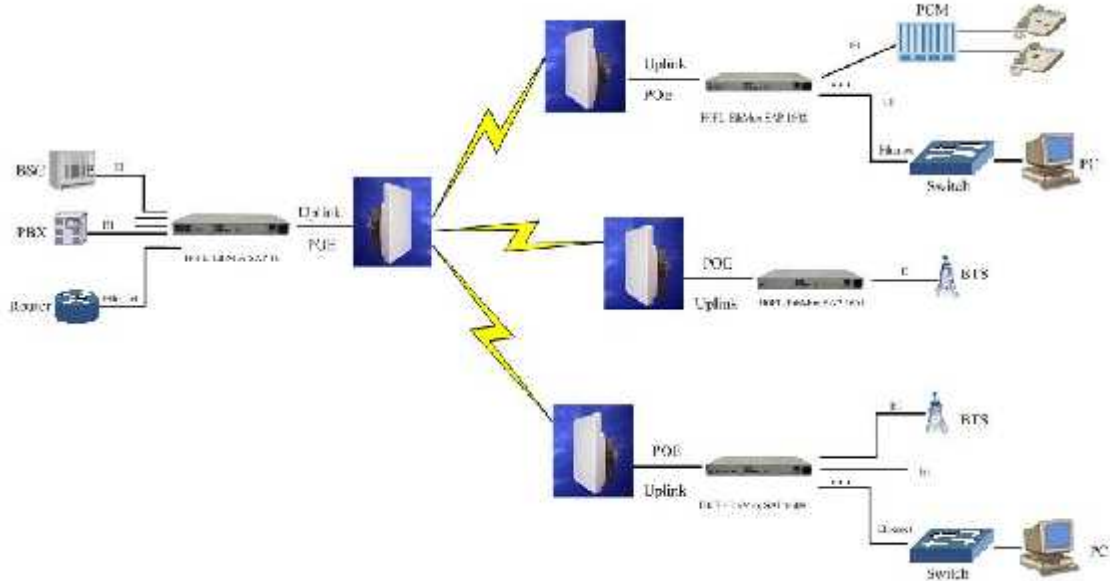
Point to multipoint application
