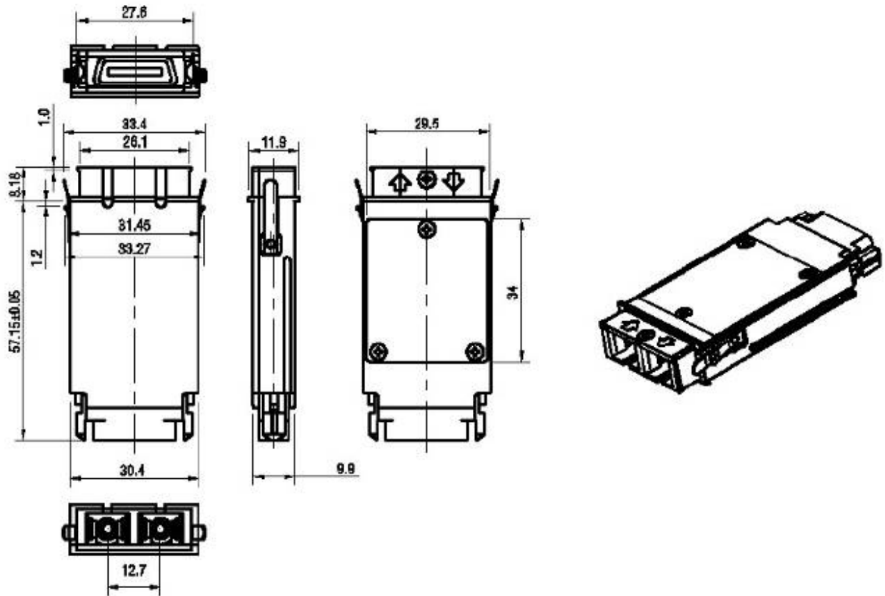
GBIC-LH
