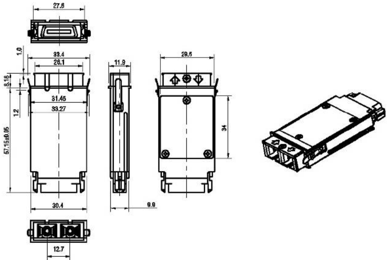
GBIC-SX
