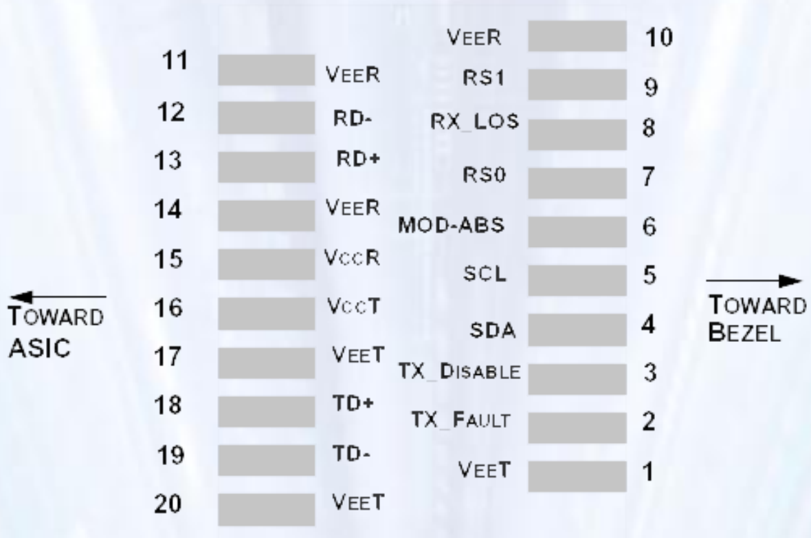
Figure 3,pins view
