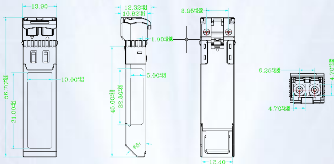
Figure 4, mechanical dimension
