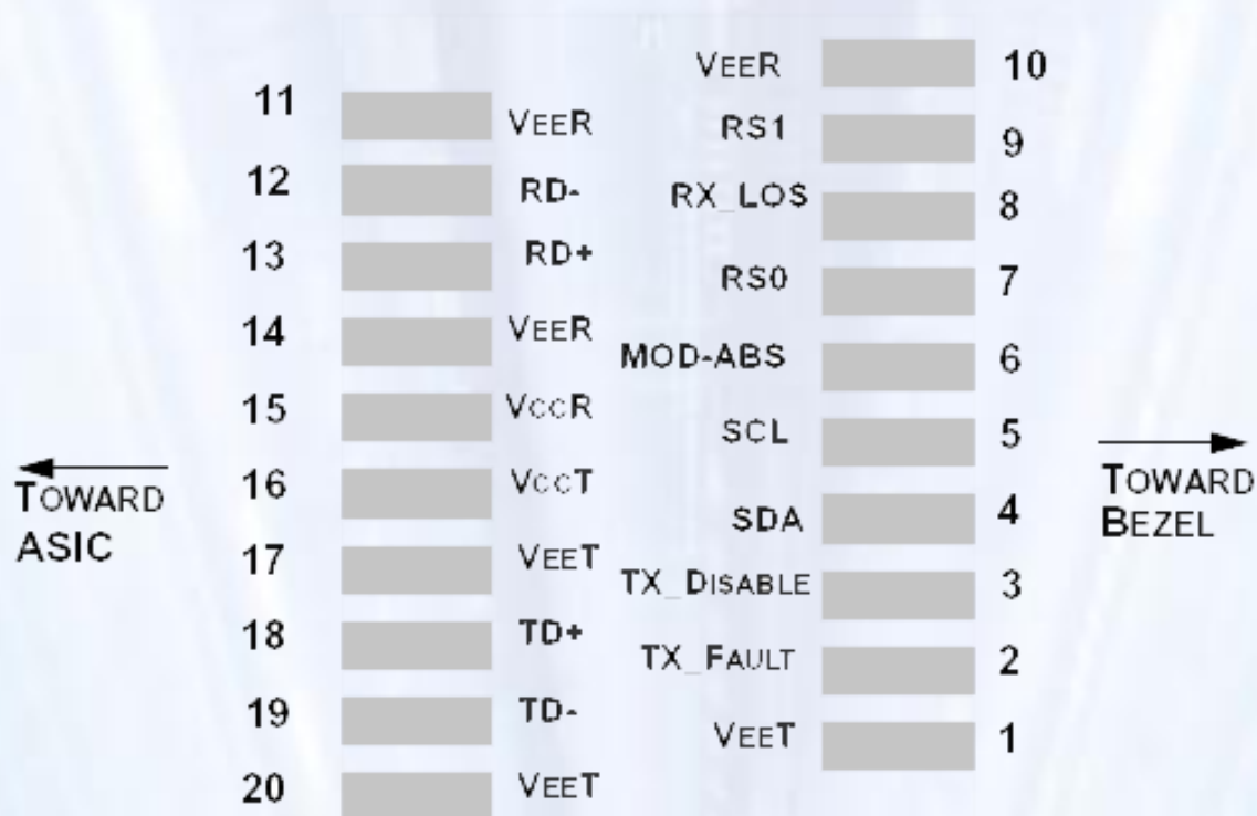
Figure 3, Pin View
