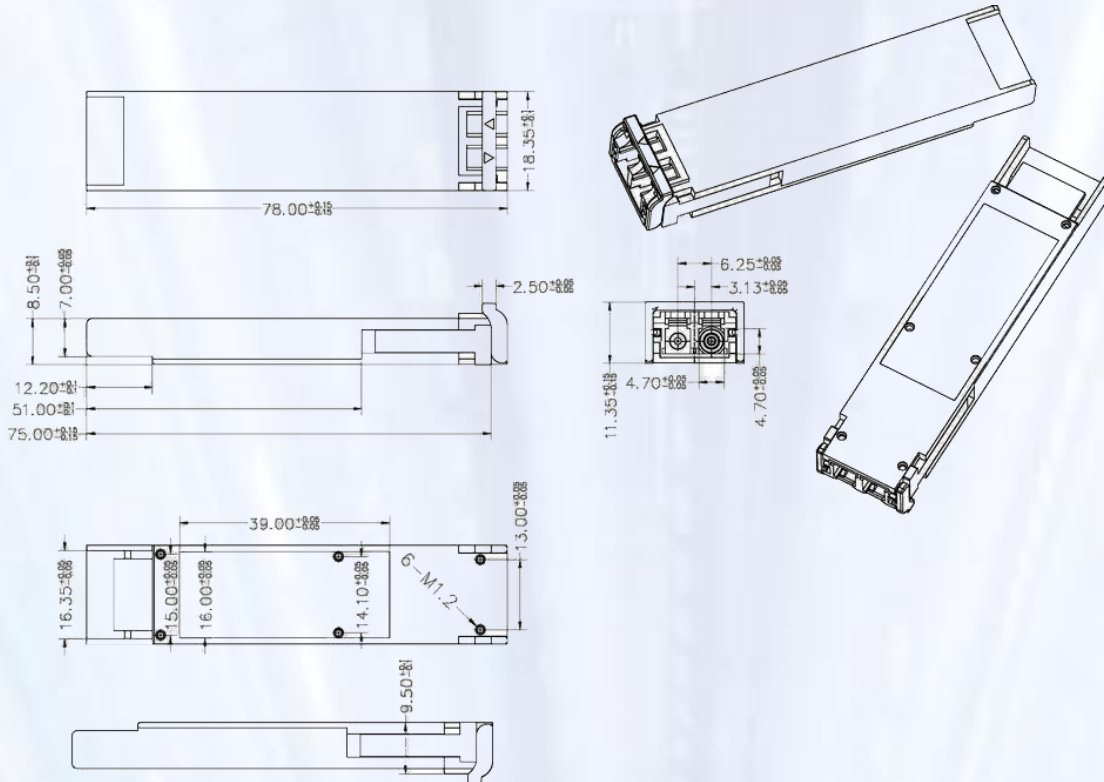
Figure 4,mechanical dimension
